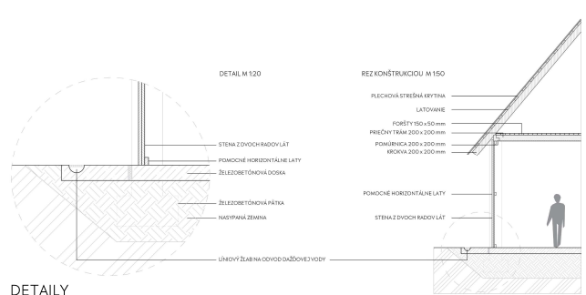
DETAILY
