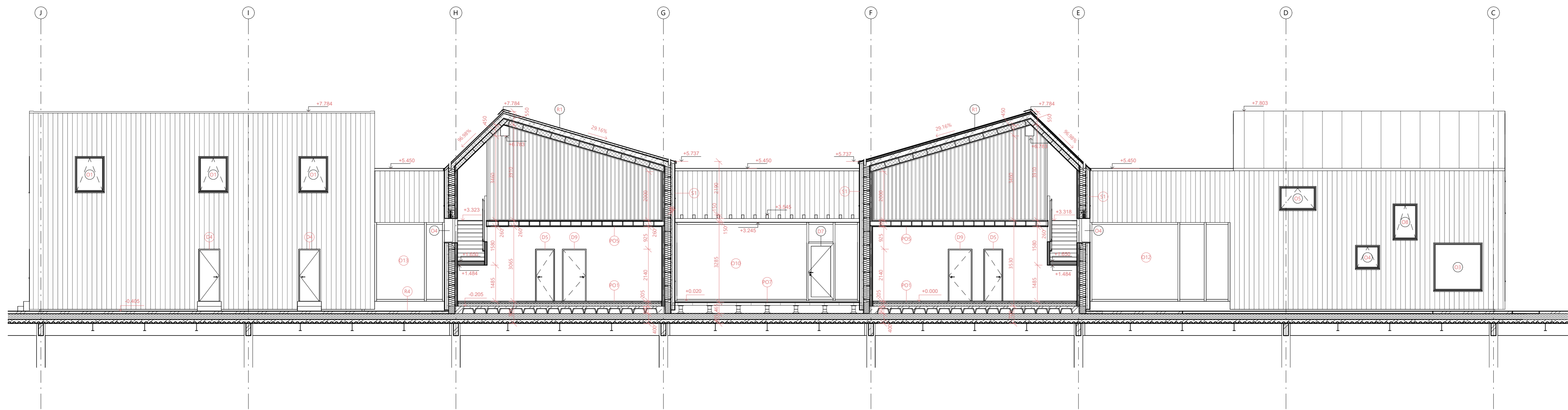
REZ C-C'
