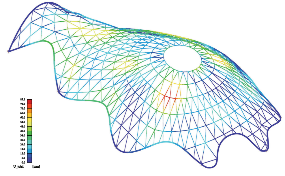
3D DEFORMACE
